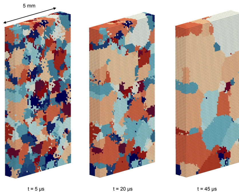
Fig.: Metal grain growth over time due to solid state phase transformation. Simulated with Peridynamics.
